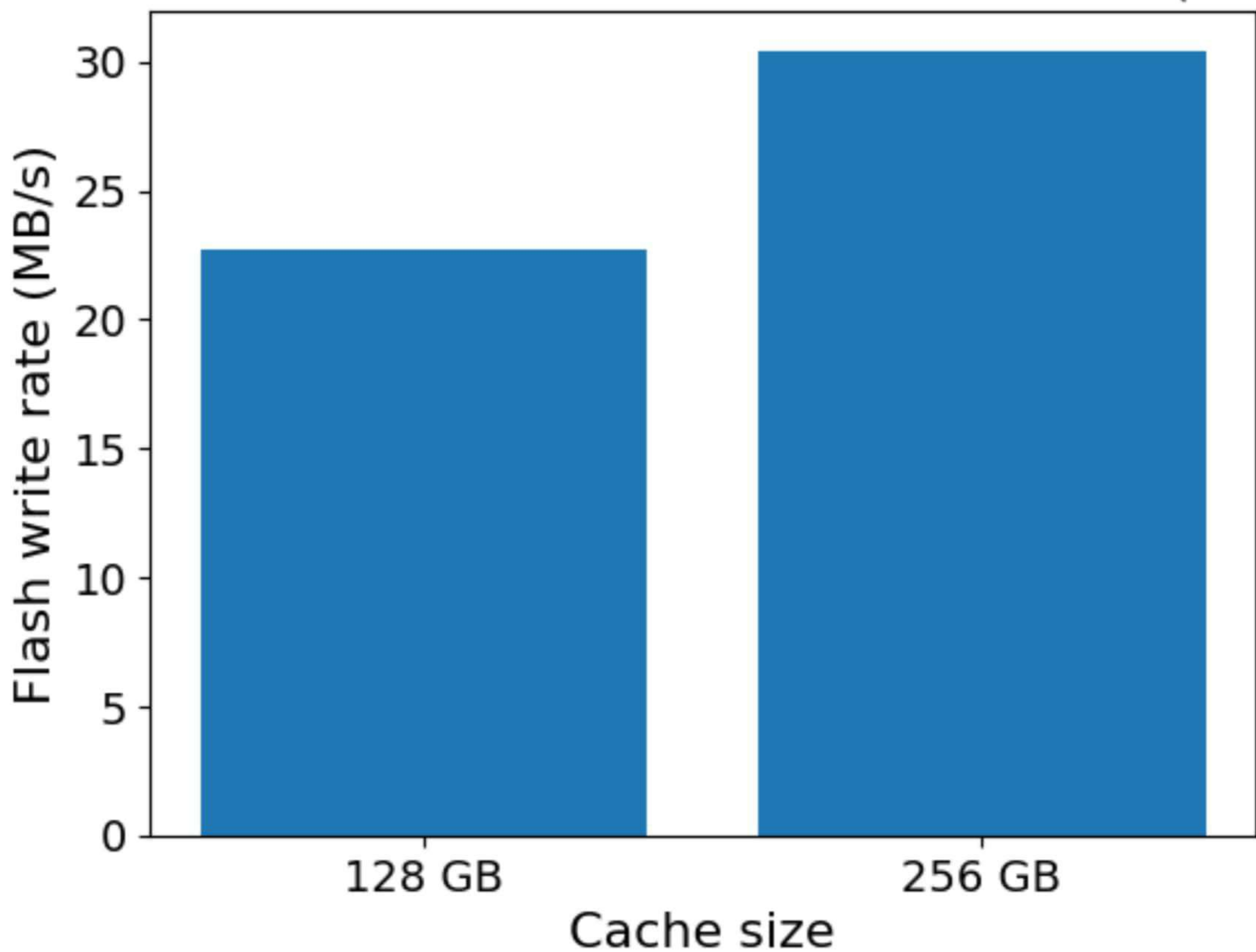
Effect of cache size on flash write rate (LRU)
